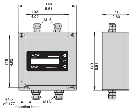
FC100-FH (surface mounted housing)
