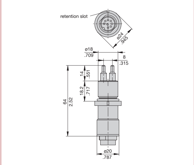
This is a metric design and millimeter dimensions take precedence (mm/inch)
